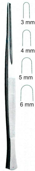
Partsch 170 mm TI-1675 3mm TI-1676 4mm TI-1677 5mm TI-1678 6mm
